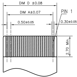
APPLICABLE FPC/FFC GENERAL TOLERANCE ±0.05 THICKNESS 0.30±0.03
